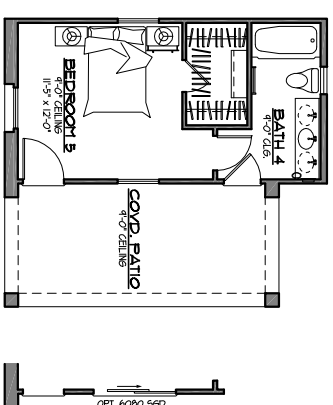
OPTIONAL DETACHED GARAGE OPT. A - BEDROOM 3/BATH 4
